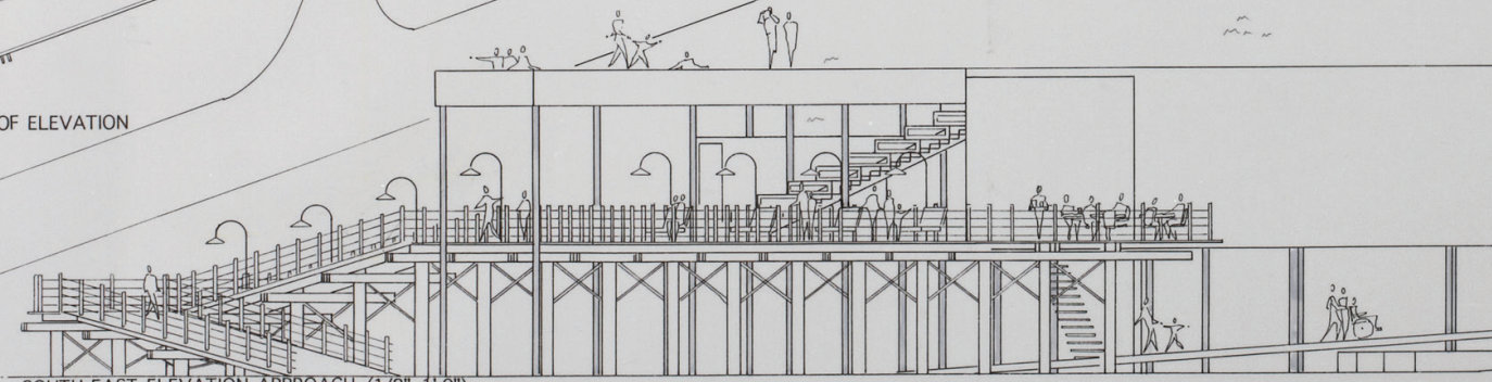
SOUTH-EAST ELEVATION APPROACH (1/8"=1'-0")
