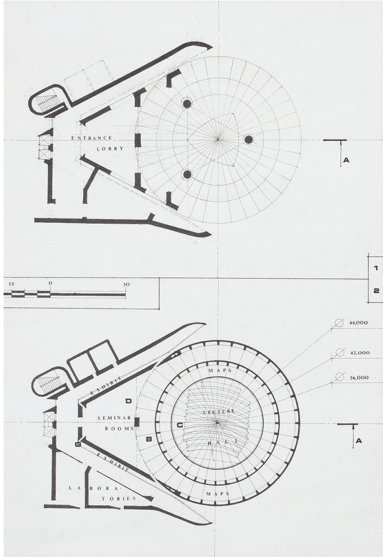
on the point ±0.000 = plan on the point 51.000 SCALE OF FEET
