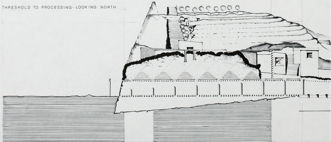
SITE SECTION
