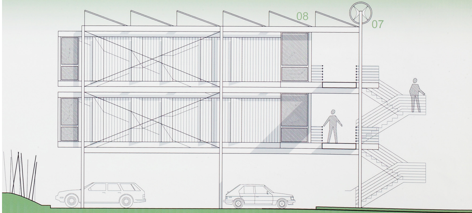
south (gulf) elevation
